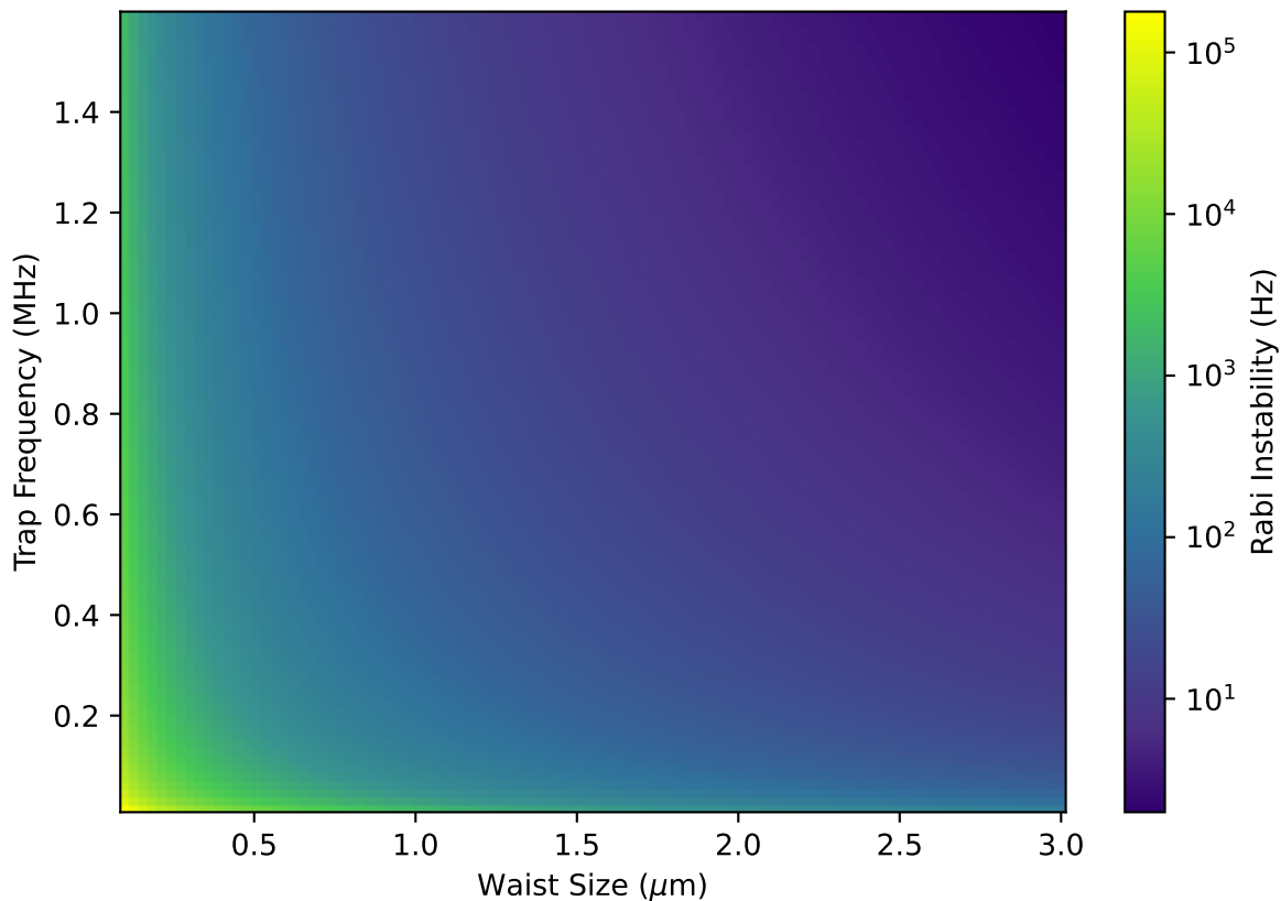
Rabi Frequency Deviation when T \ll \omega
